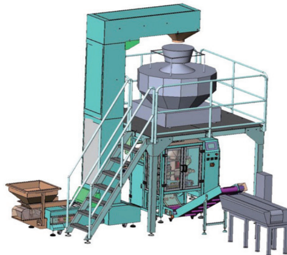
PM-430-S2 with 14 heads scale system For high speed application
